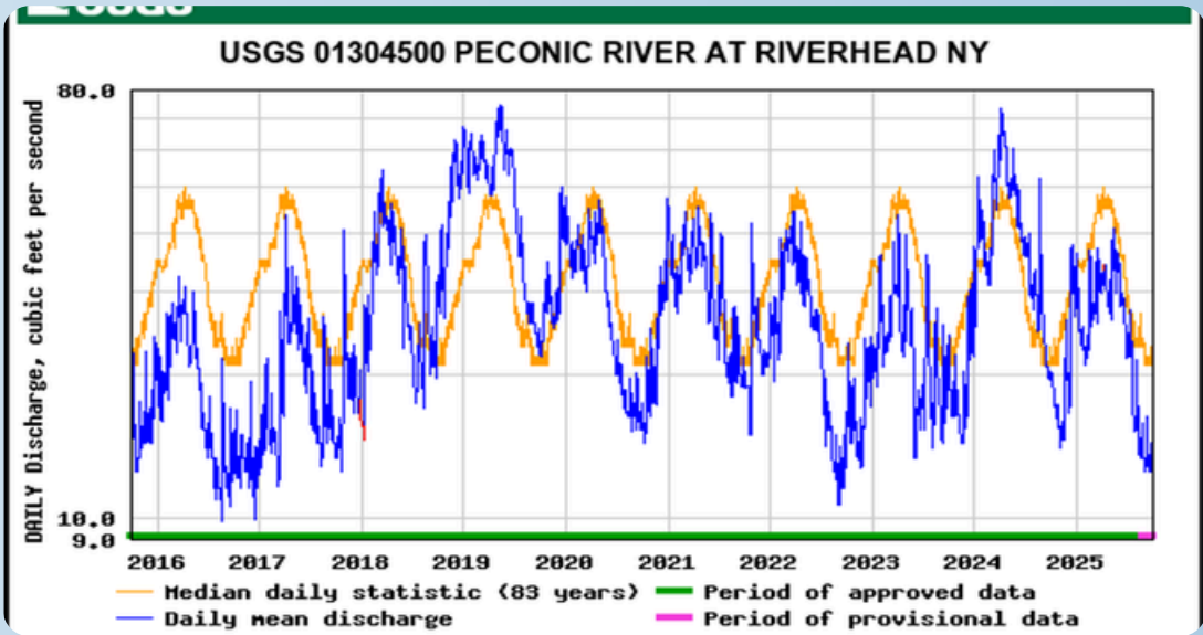
Source: https://nwis.waterdata.usgs.gov/ny/nwis/dv/?ts_id=104691&format=img_stats&site_no=01304500&begin_date=20151001&end_date=20250930
