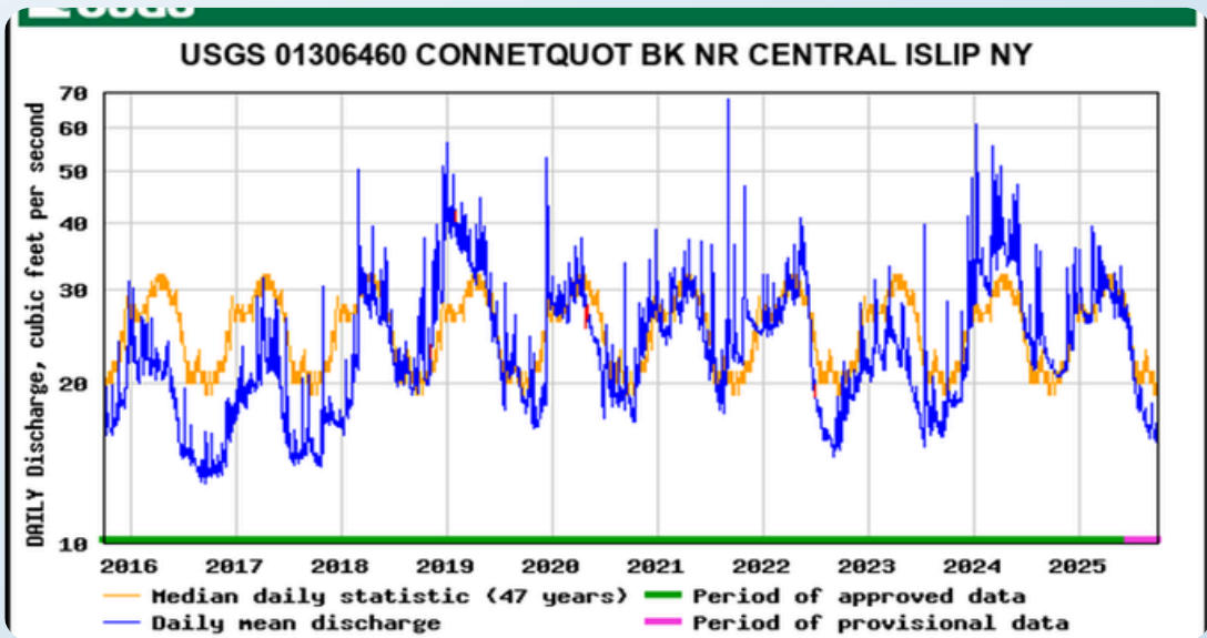
Source: https://nwis.waterdata.usgs.gov/ny/nwis/dv/?ts_id=226479&format=img_stats&site_no=01306460&begin_date=20151001&end_date=20250930
